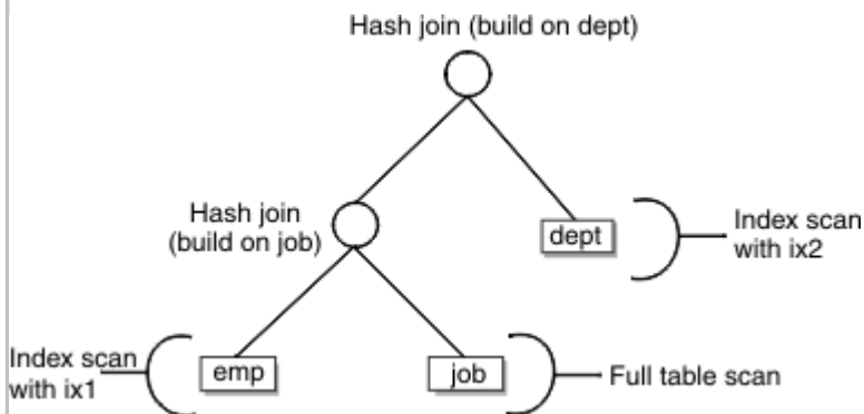
Figure 60. Possible query plan with directives
