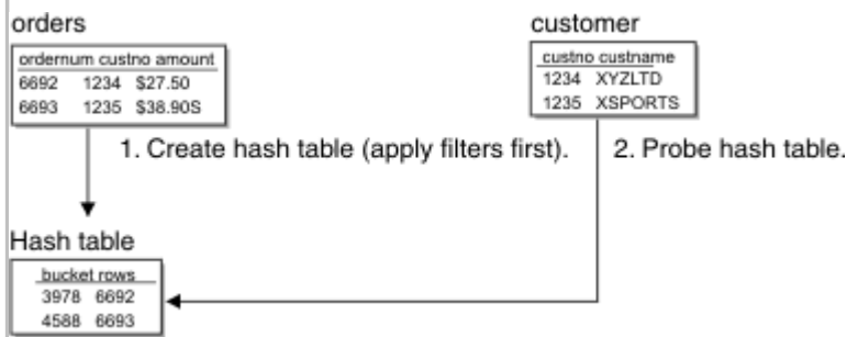
Figure 40. How a hash join is executed
