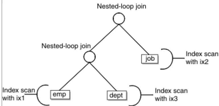
Figure 59. Possible query plan without directives
