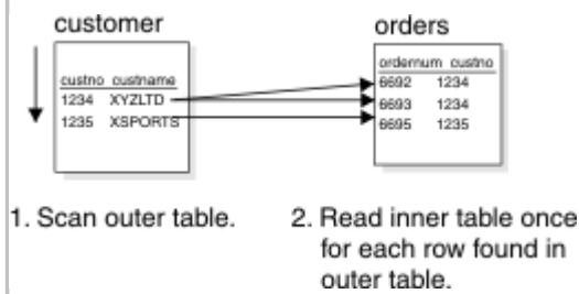
Figure 39. Nested-loop join
