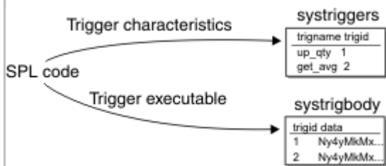
Figure 57. Trigger information stored in system catalog tables
