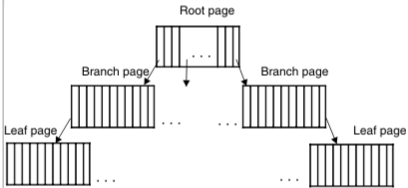
Figure 26. B-tree structure of an index
