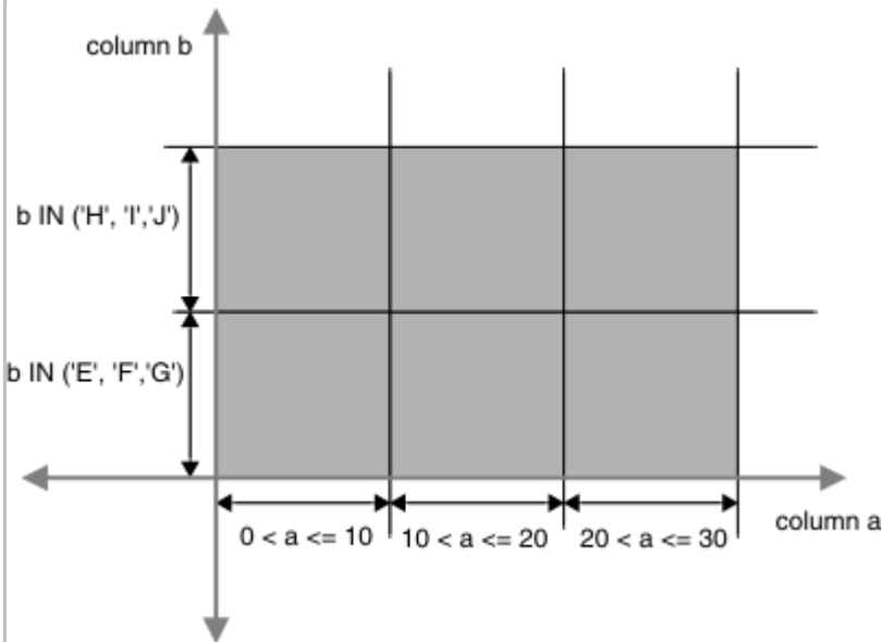
Figure 38. Schematic example of nonoverlapping fragments on two columns
