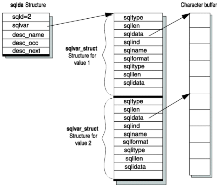
Figure 76: Schematic that shows sqlda structure for two values on page 432 shows the column data in the sqldata fields in a single data buffer. This data can also be stored in separate buffers.
