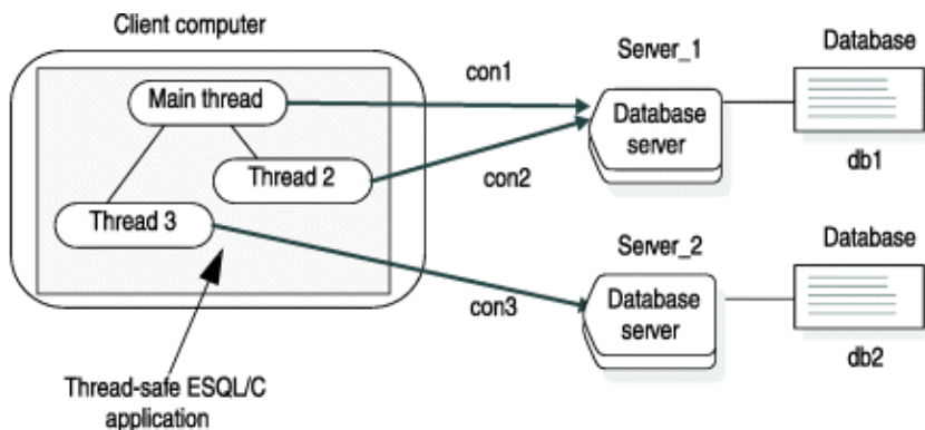
Figure 72. Concurrent connections in a thread-safe ESQL/C application
