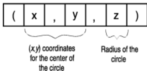
Figure 52. External Format of the circle Opaque data type
