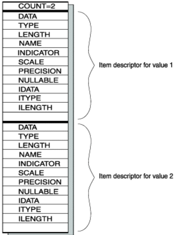
Figure 75. Schematic that shows system-descriptor area for two values
