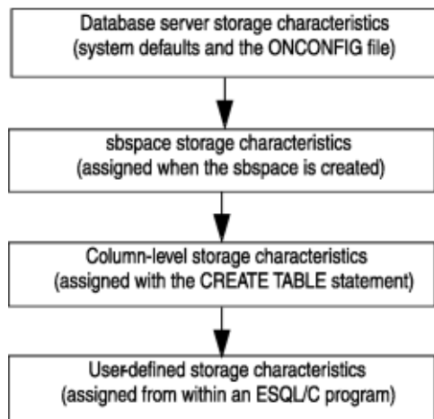
Figure 35. Inheritance hierarchy for storage characteristics
