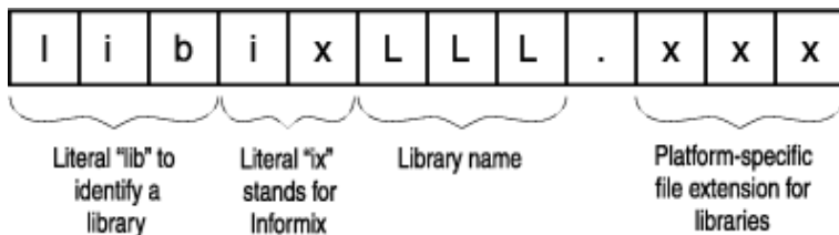
Figure 71. Format of the Informix® shared-library name
