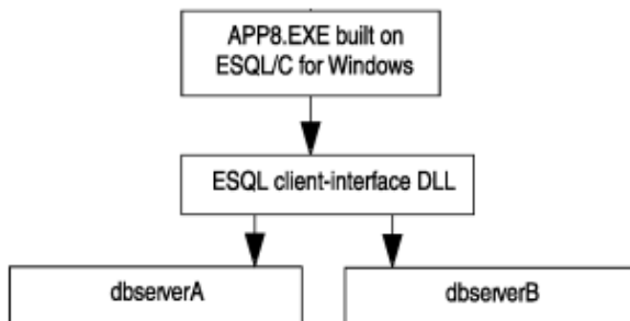
Figure 70. One application that uses connections to more than one database server at the same time
