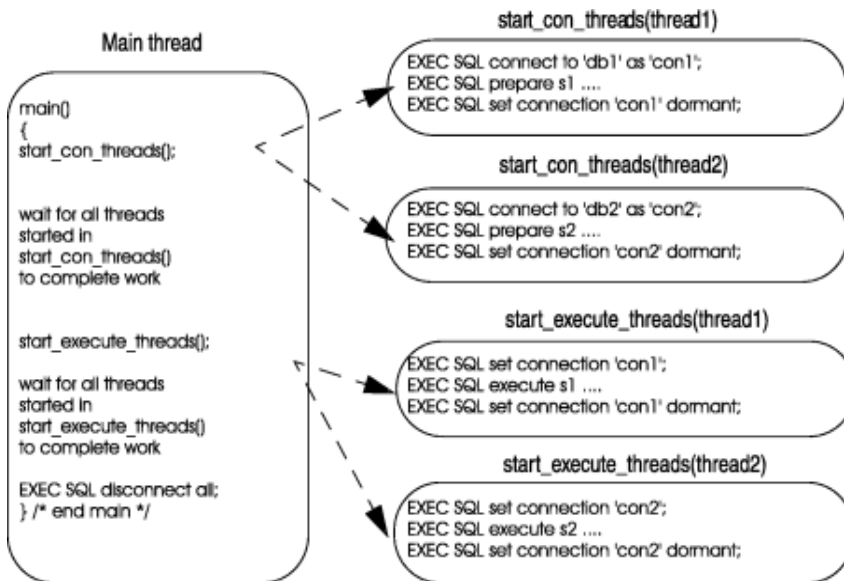
Figure 73. Using prepared SQL statements across threads
