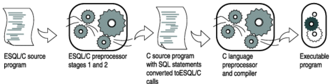
Figure 15. Relationship between Informix® ESQL/C and C
