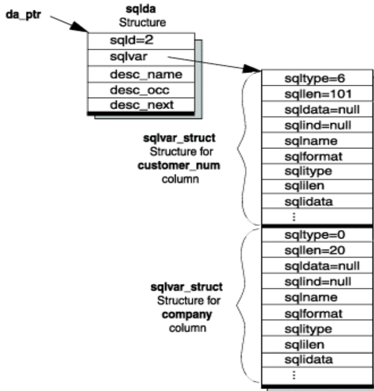
Figure 79. Sample sqlda Structure for Two Columns
