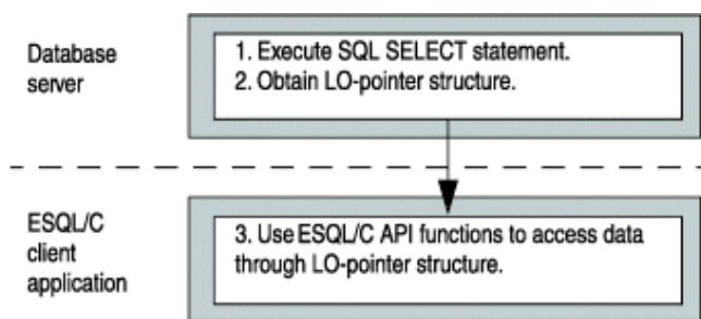
Figure 37. Transferring smart- large-object data from database server to client application
