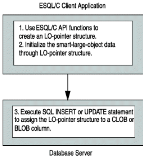
Figure 36. Transferring smart-large-object data from client application to database server
