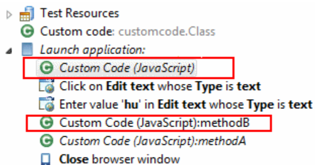
Figure 12. Custom code added as a test step in a Web UI test
